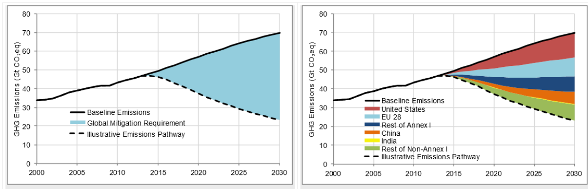
Figure 2: Indicative emissions reduction requirements to 2030 (for 2°C mitigation pathway) 22
