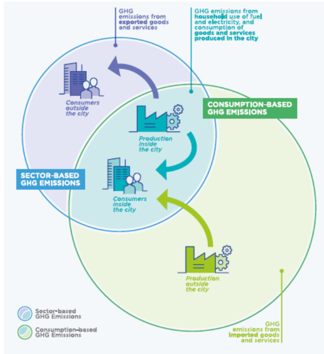
Figure 4: Illustration of Scopes 1, 2 and 3 (Consumption) Emissions, (C40, 2018)
